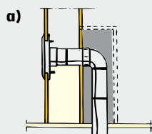
Fig. 6 Wall mounting
